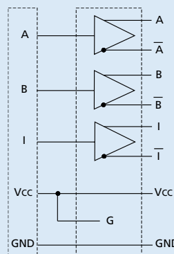
Connection diagram
