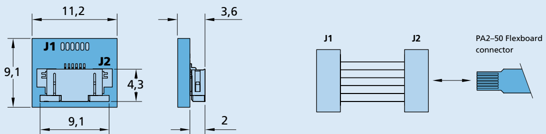
Connector J1 – Solder Pads J2 – Molex 52475-0690
