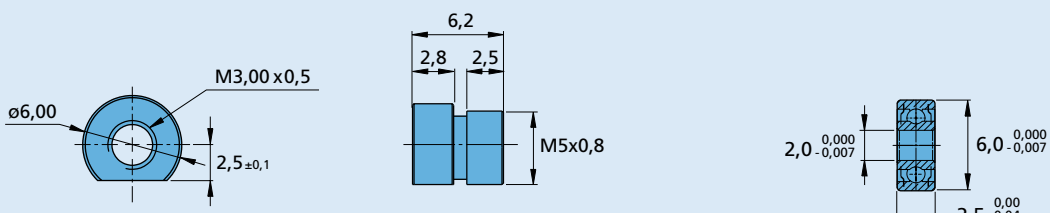
Nut Part No. 2.8000.90.531, Self-lubricating synthetic material
